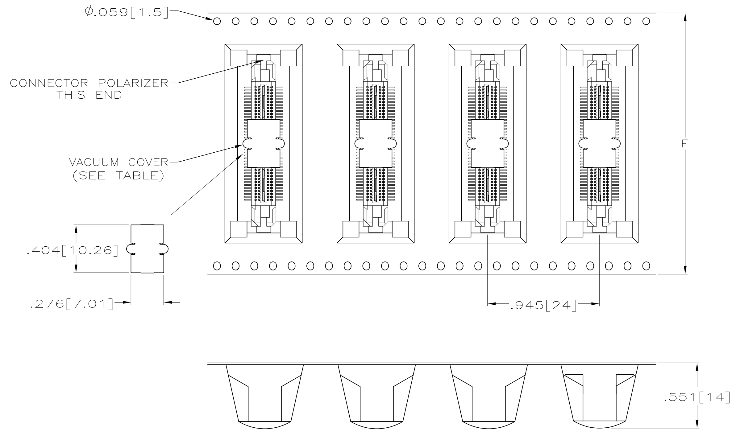
PACKAGING DETAIL SCALE 2:1 DIMENSIONS ARE FOR REFERENCE
